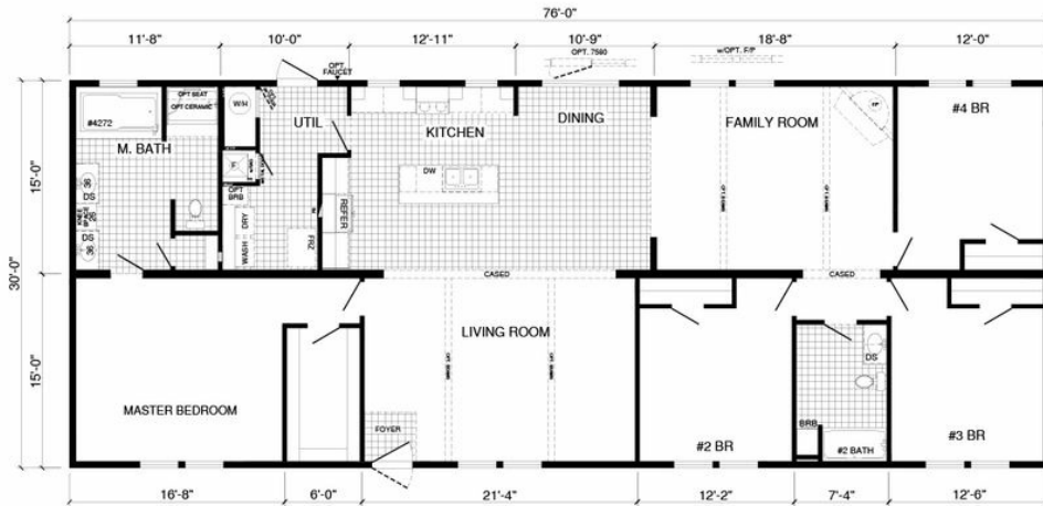
MODEL: MANORVIEW II WL-8023B 32'-0" x 80'-0" 2,280 Sq.Ft 4 Beds 2 Baths
