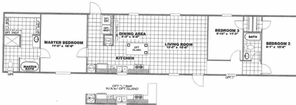
MODEL # VAL16763S DRAWING # 35S289 16' x 76' VALUE
