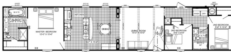
MODEL BRB-1833 3-BEDROOM / 2-BATH 16' x 82' - Approx. 1170 Sq. Ft.
